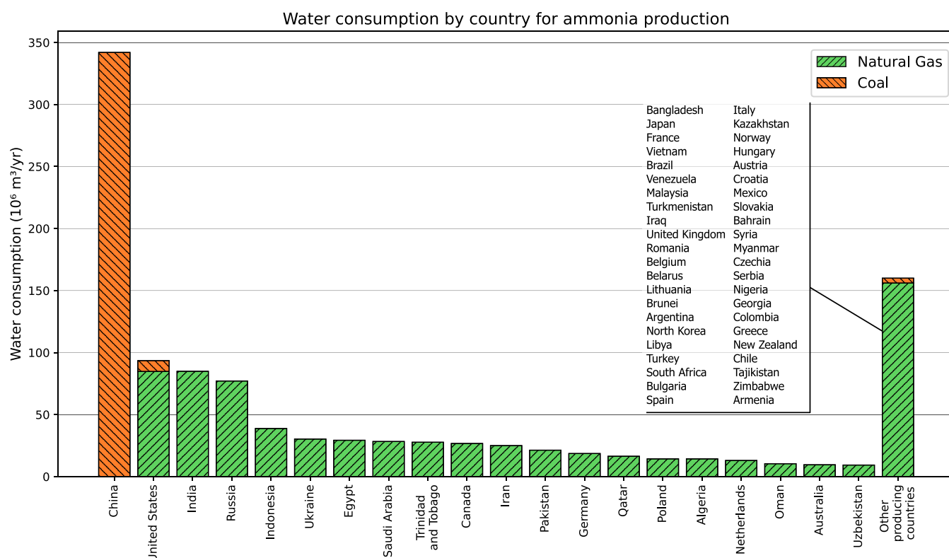
Figure 2. Estimated direct water consumption for ammonia production by country ( \text{million m}^3 \text{ yr}^{-1} ). Bars are colored according to the share of facilities fed by natural gas (steam methane reforming-based ammonia production) (green) and coal gasification-based ammonia production (orange). Countries are sorted by direct water consumption, with only the top 20 producers shown individually. The remaining countries are aggregated under “Other producing countries”.
